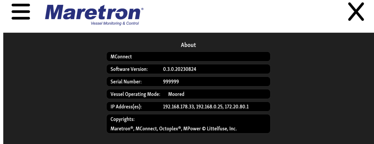
Figure 11 – About Dialog
