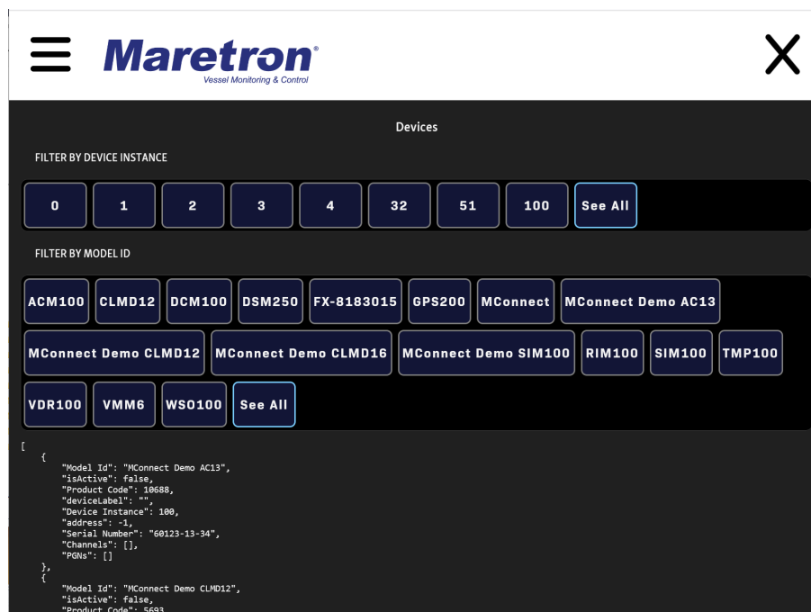
Figure 12 – Devices Dialog
