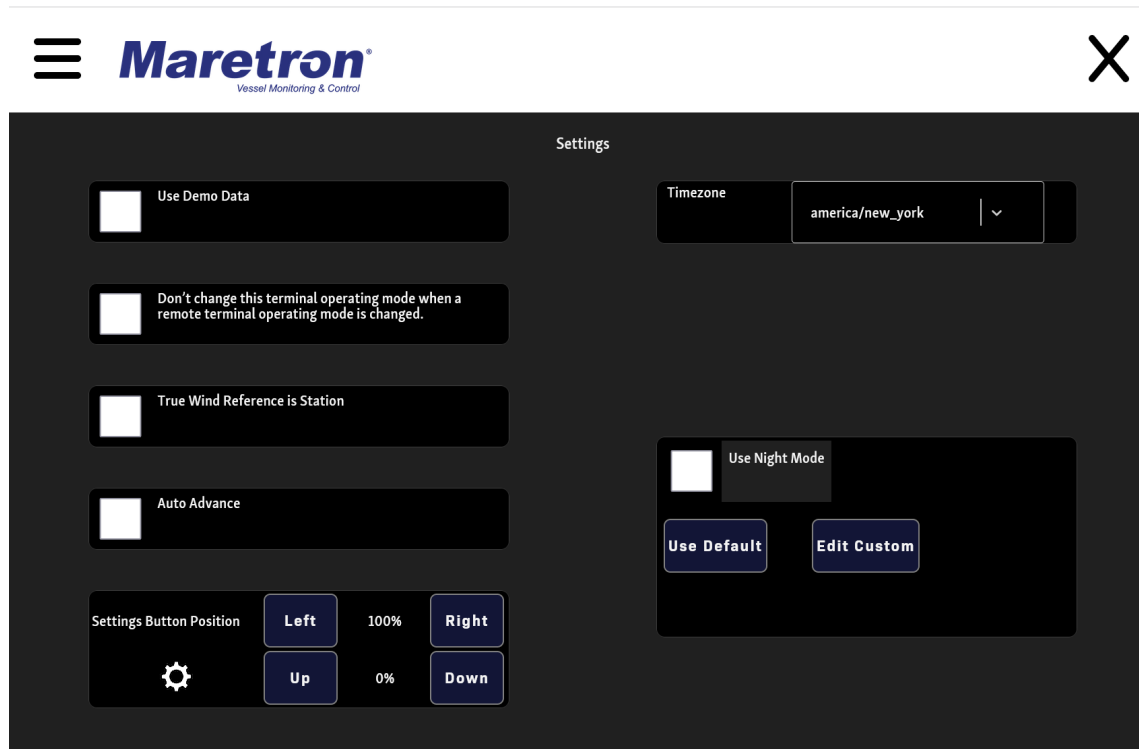
Figure 6 – Settings Dialog
