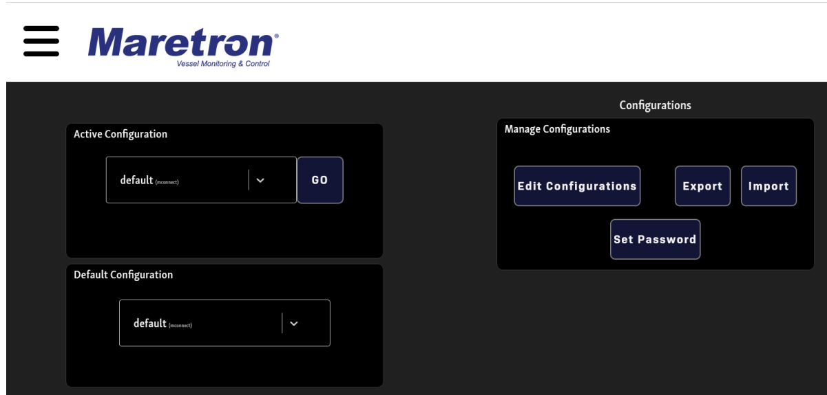
Figure 7 – Configuration Dialog
